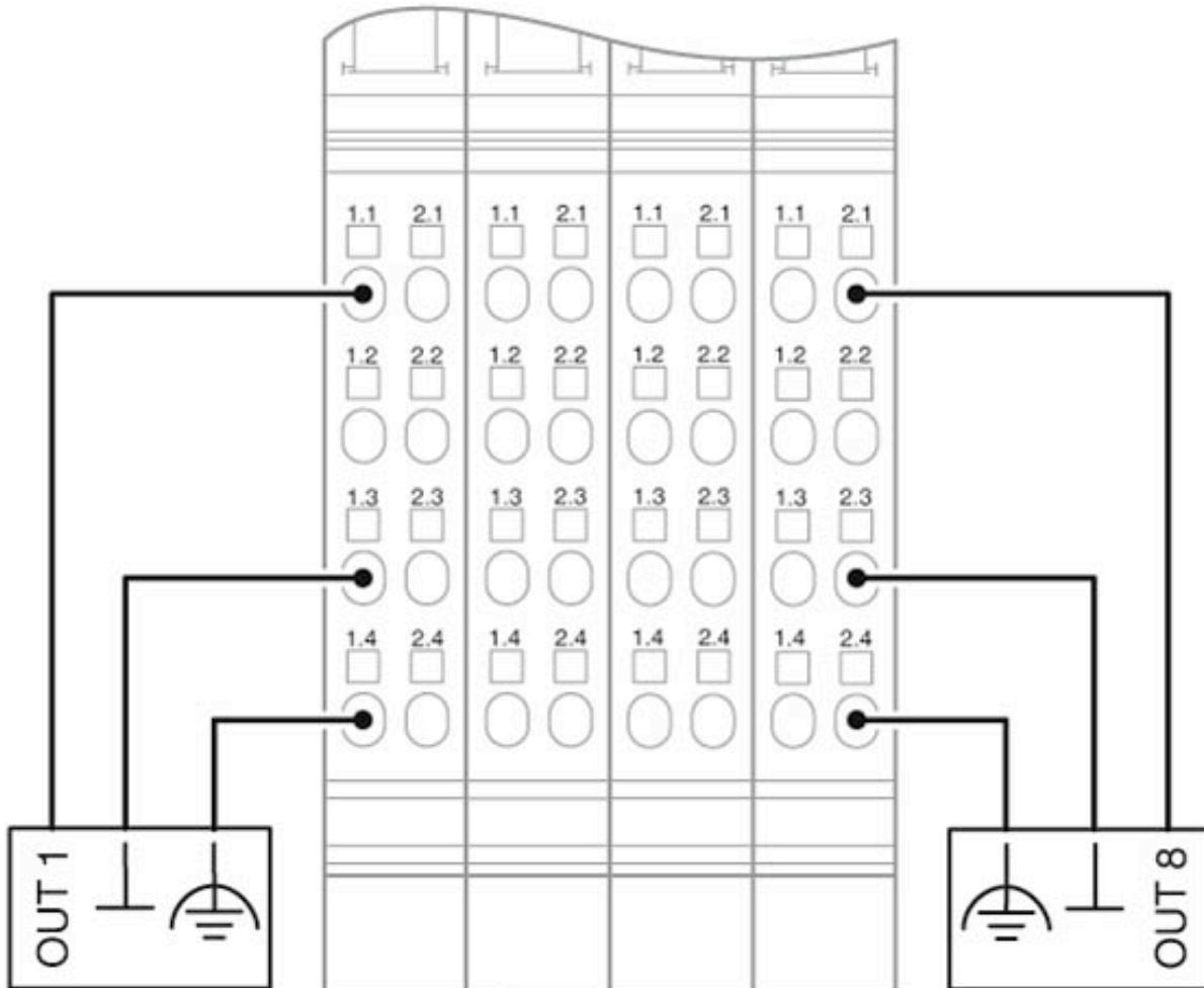
Connection diagram
